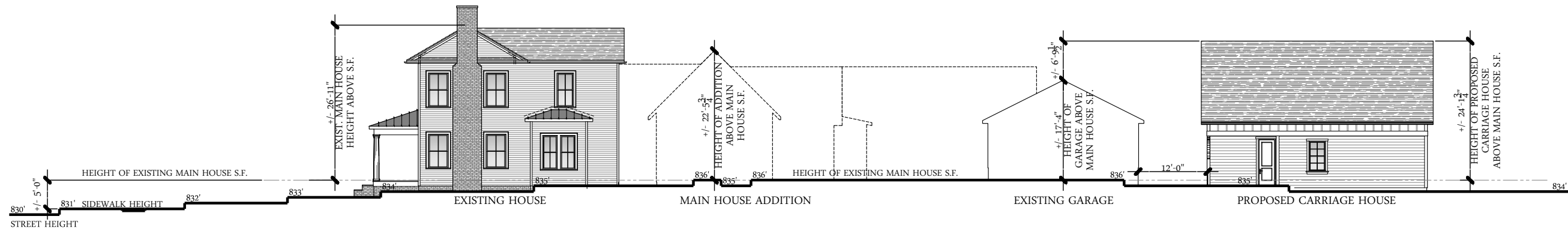
SITE ELEVATIONS (FROM RIGHT SIDE OF PROPERTY)
