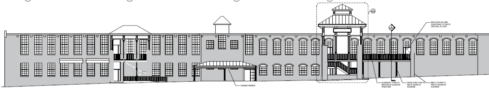
1 SOUTH BUILDING ELEVATION - NEW WORK SCALE 1/8" = 1'-0"
