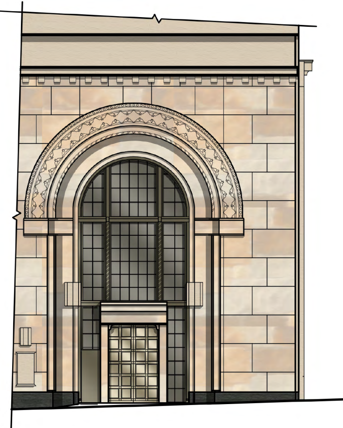
SOUTHEAST ELEVATION
